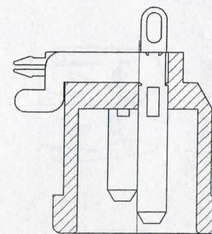
SEC B-B
